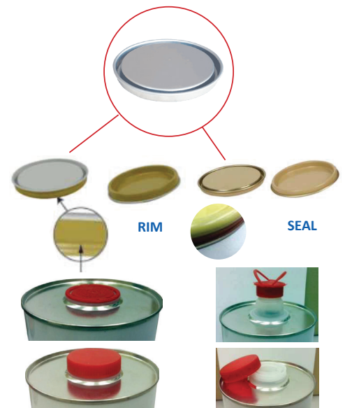
CONICAL DRUM, WITH PLACE FOR PLASTIC INSERT
